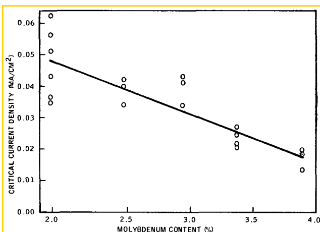
Fig. 2. Critical current densities obtained from potentiodynamic scans at 600 mv/hr in argon-saturated 0.1N hydrochloric acid on the 16.6% Cr-13.5% Ni steels.
